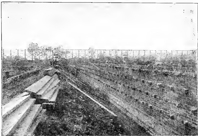
OUTSIDE WALL, READY FOR CONCRETE BACKING.
